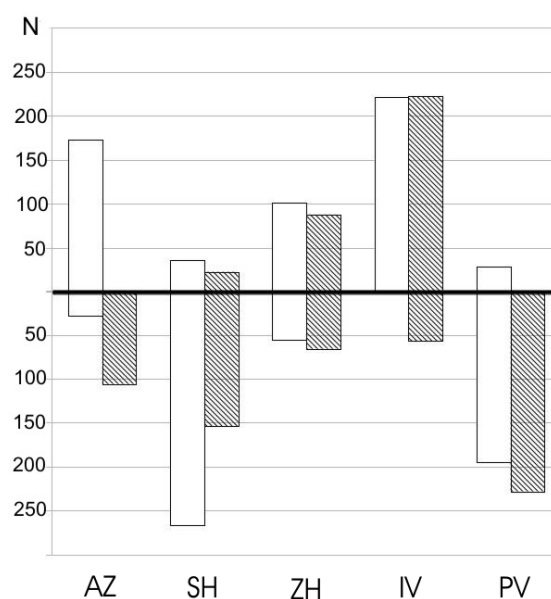
Fig. 2. Individual examples of the 'pattern' of saccade responses in subjects AZ, SH, ZH, IV and PV. N – the number of saccade responses. The columns above the x-axis denote the number of double saccade responses, the columns under the x-axis denote the number of the single saccade responses. White columns denote the 150ms duration of the first target, shaded columns denote the 50 ms duration of the first target.
