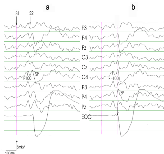
Fig. 3. Averaged EEG potential prior to the double saccade response in subject VD. a – direct averaging from the first stimulus onset (S1 arrow). S2 arrow –the second stimulus. S1 was in the left hemifield, S2 - in the right one. S1 duration - 150ms. b – backward averaging from the saccade onset (arrow on the EOG channel). Number of EEG averaging - 25.
