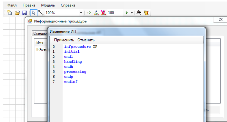
Fig.2. The form for information procedure
