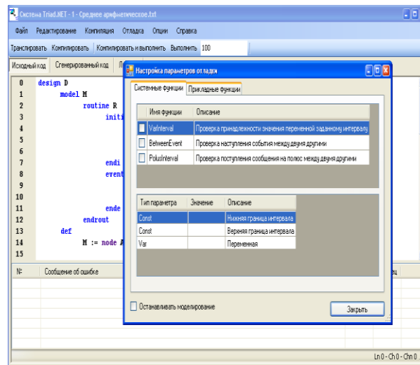
Fig. 4. Simulation model editor and information procedures for algorithm of investigation and debugging
