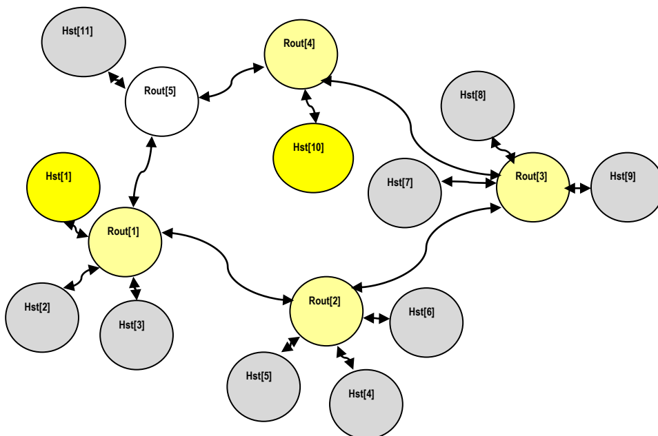
Fig. 5. Graph representation of the simulation model structure
