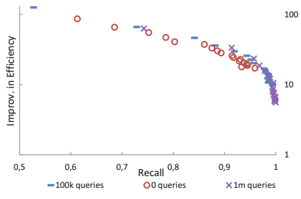
Fig. 2. The overall efficiency of the structure after applying Repair_By_Query procedure
