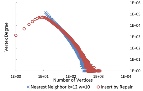
Fig. 4. Vertex Degree Distribution
