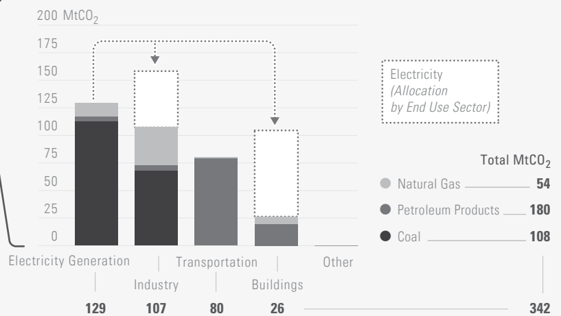
Figure 3. Decomposition of historical energy-related CO 2 Emissions, 1990 to 2010
