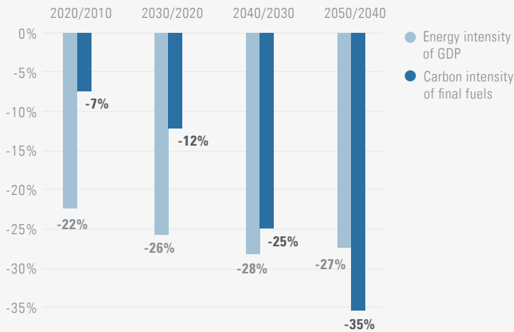
Figure 6.7. Decadal percent change in Energy/GDP and CO 2 /Energy for the 15 DDPs, 2010 to 2050
