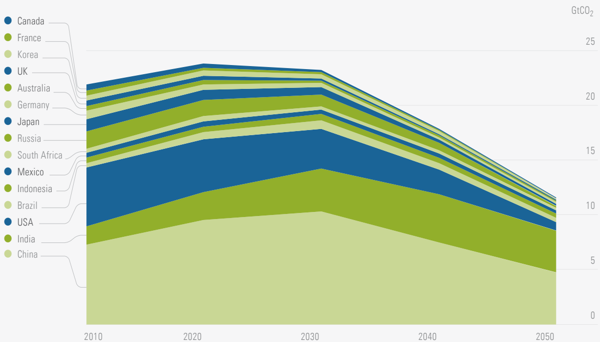
Figure 6.3. Energy-related CO 2 emissions reduction trajectories in the 15 DDPs
