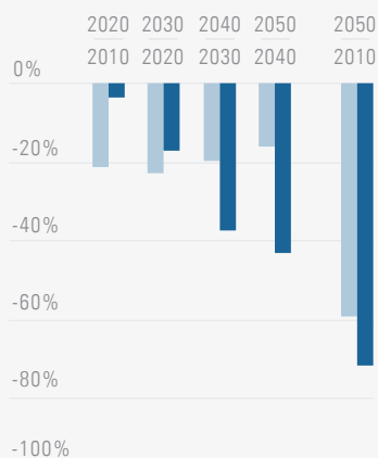
Figure 3.2. Decadal and cumulative percent change in Energy/GDP and \text{CO}_2/\text{Energy} for the IPCC 2^\circ\text{C} scenarios, 2010 to 2050
