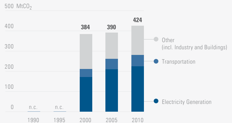
Figure 2. Decomposition of historical energy-related CO 2 Emissions, 1990 to 2010
