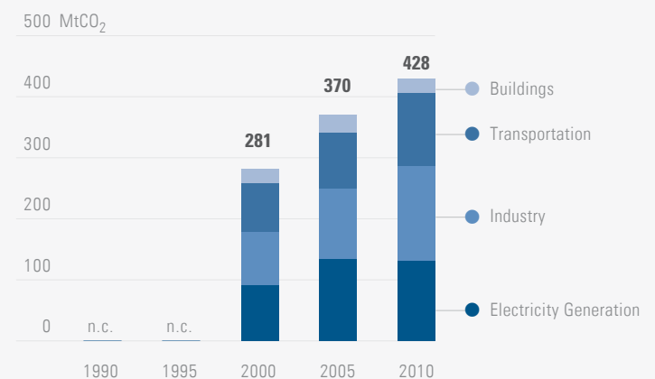
Figure 3. Decomposition of historical energy-related CO 2 Emissions, 1990 to 2010
