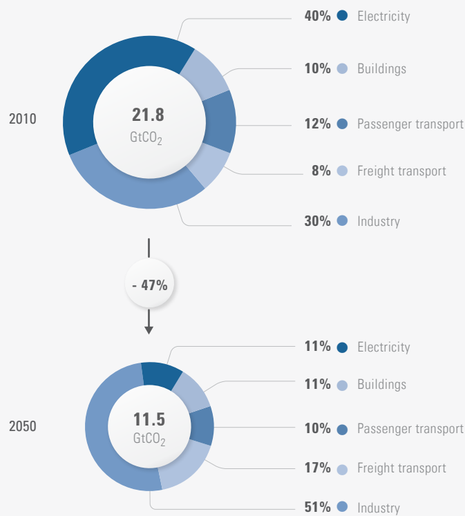
Figure 6.8. Sectoral shares of CO 2 -energy emissions, 2050 compared to 2010
