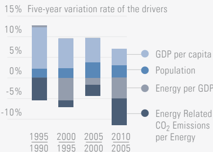
Figure 2. Decomposition of historical energy-related CO 2 Emissions, 1990 to 2010
