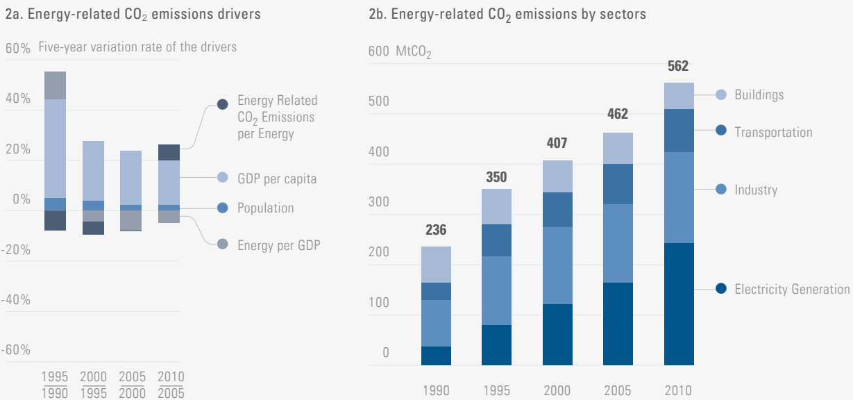
Figure 2. Decomposition of historical energy-related CO 2 Emissions, 1990 to 2010
