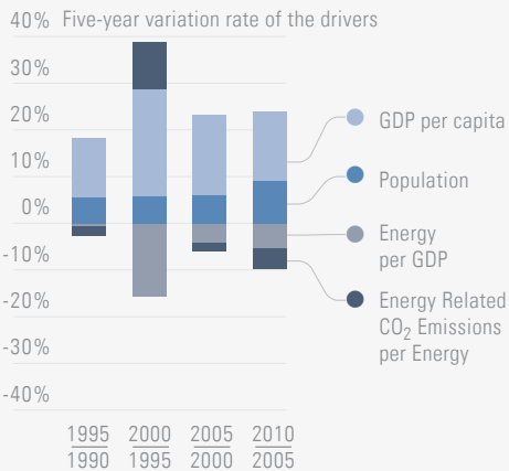
Figure 3. Decomposition of historical energy-related CO 2 Emissions, 1990 to 2010
