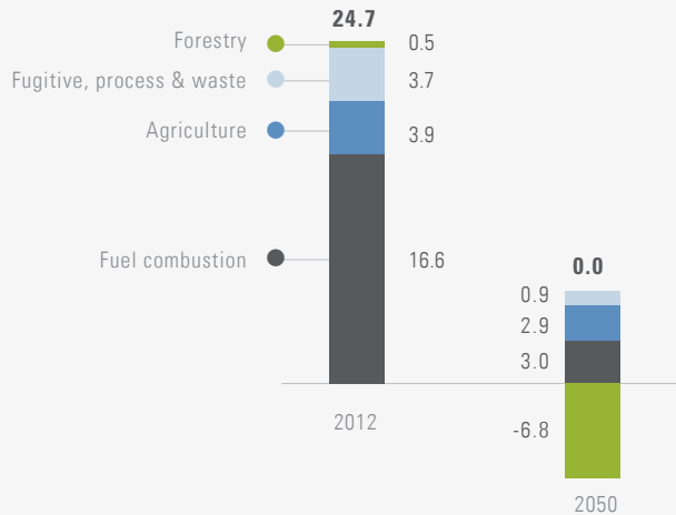
Figure 8. Greenhouse gas emissions per capita by sector and source, tCO 2 eq per capita, 2012 and 2050
