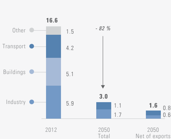
Figure 8. Greenhouse gas emissions per capita by sector and source, tCO 2 eq per capita, 2012 and 2050
