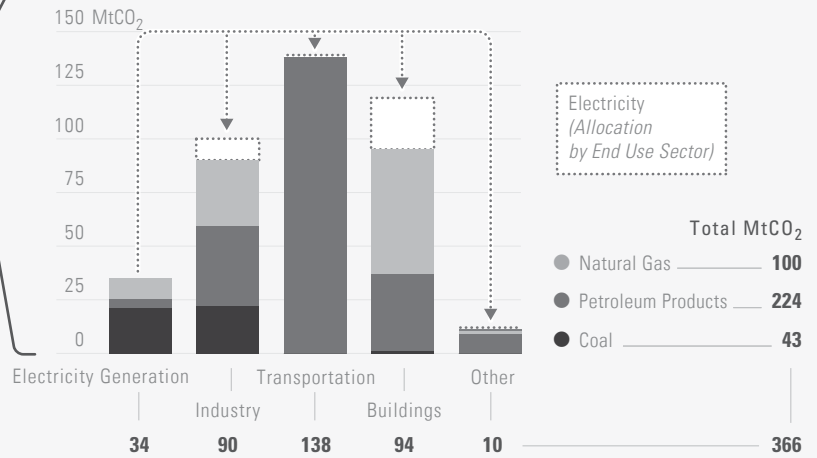
Figure 2. Decomposition of historical energy-related CO 2 Emissions, 1990 to 2010
