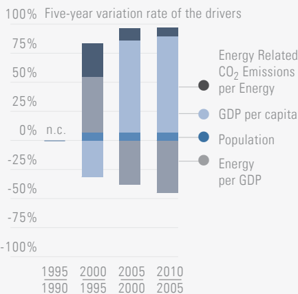
Figure 3. Decomposition of historical energy-related CO 2 Emissions, 1990 to 2010
