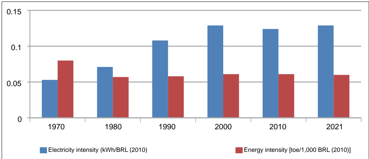
Graph 5: Energy and Electricity Intensity, Brazil
