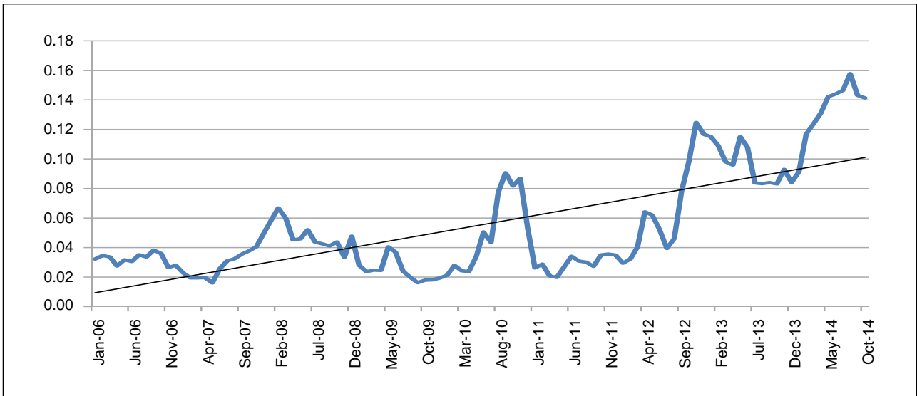
Graph 7: Electricity Emission Factor in Brazil (tCO 2 /MWh)
