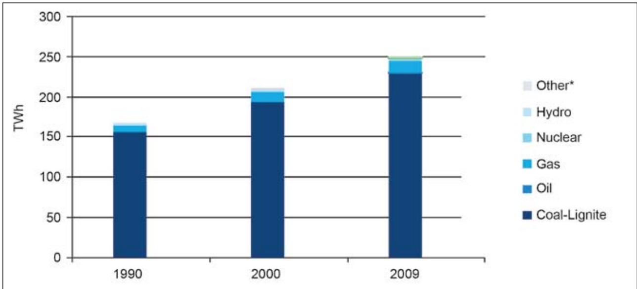
Graph 11: Power Generation by Source, South Africa
