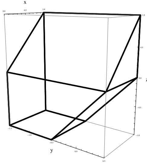
FIGURE 5. Polytope D_1E_uD_2D_1(a) for a = (0, -1, -1) and u = (0, -1/2, 0)
