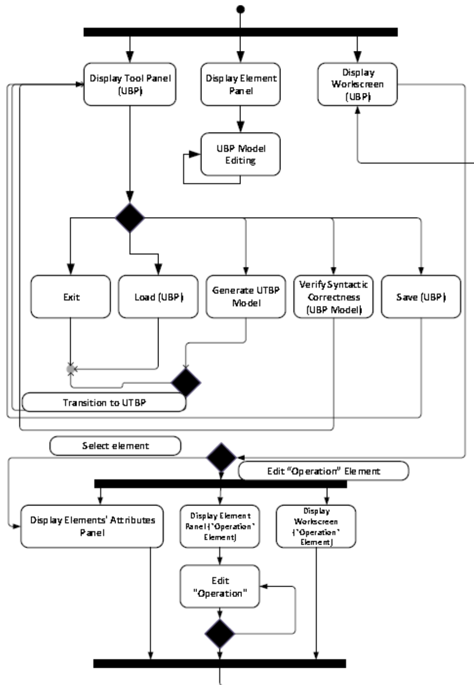
Figure 3. UBP Model Interaction Activity Diagram
