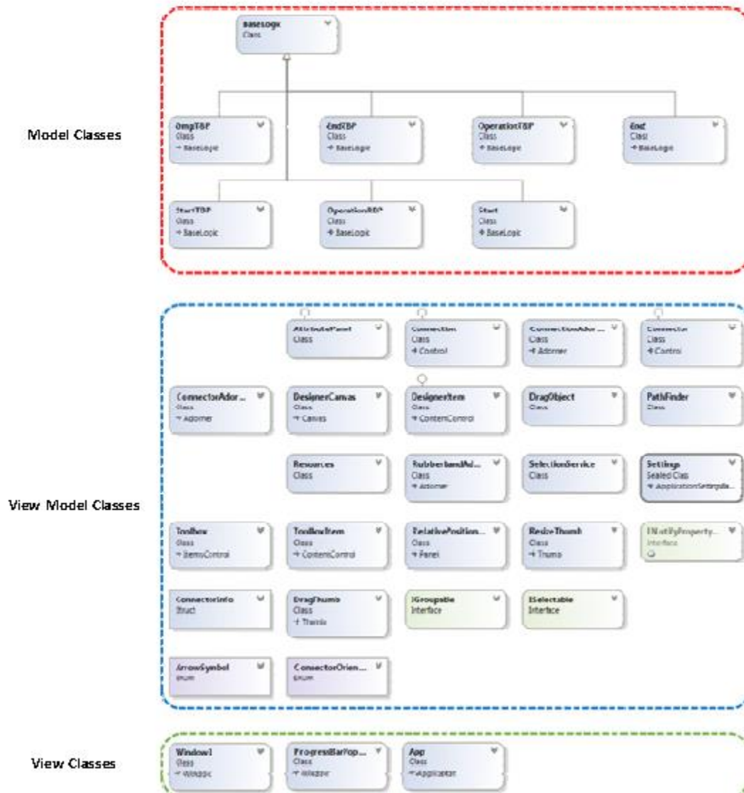
Figure 6. Class Diagram
