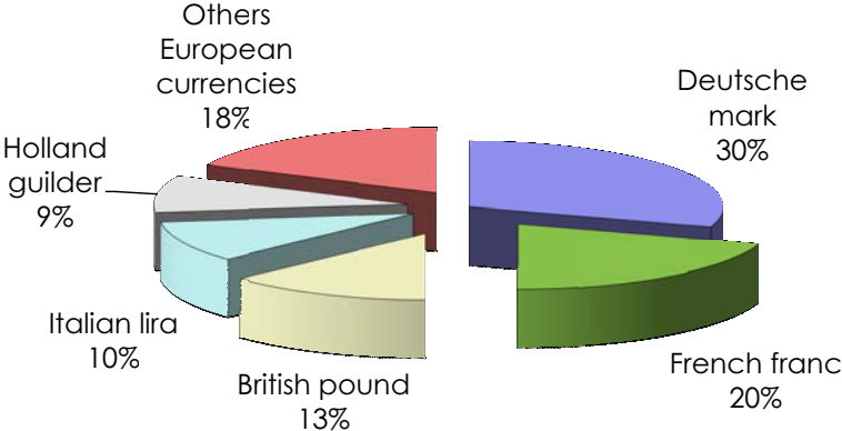
Exh. 1.5. Ultimate “basket” of ECU, 1988
