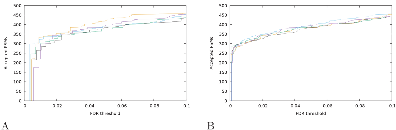
Figure 3. Average target-decoy competition reduces decoy-induced variance. (A) Plots of the number of accepted PSMs ( y -axis) as a function of FDR threshold ( x -axis), for searches against databases of varying size. Each series is generated by searching a different, randomly shuffled decoy database. (B) Similar to panels (A), except that each of the five series in the plot corresponds to FDR estimates from aTDC, using five decoys per target.
