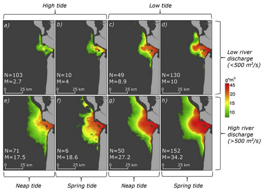
Fig. 4. SPM surface plume extension for multiple environmental conditions; N is the number of images used to compute each composite product; M represents the mass of the plume in 10^3 \times t .
