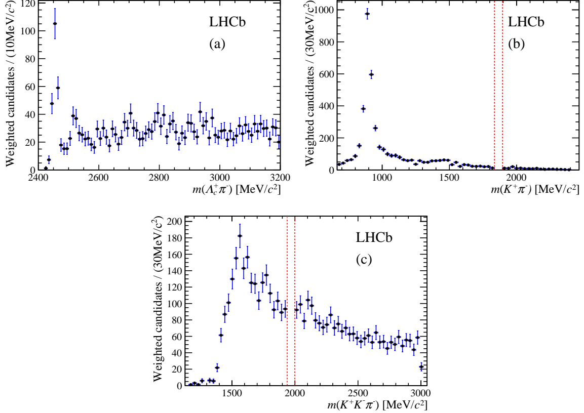
Figure 4: Invariant mass distributions of (a) the \Lambda_c^+ \pi^- , (b) K^+ \pi^- , and (c) K^+ K^- \pi^- systems in the \Lambda_b^0 \rightarrow \Lambda_c^+ K^+ K^- \pi^- signal channel, for the background-subtracted data. The red dashed vertical lines indicate the veto mass intervals for \bar{D}^0 mesons in the K^+ \pi^- distribution, and D_s^- in the K^+ K^- \pi^- distribution.
