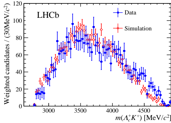
Figure 3: Invariant mass distributions of \Lambda_c^+ K^+ candidates in the \Lambda_b^0 \rightarrow \Lambda_c^+ K^+ K^- \pi^- signal channel for the simulation (red line) and the background-subtracted data (blue points with error bars).
