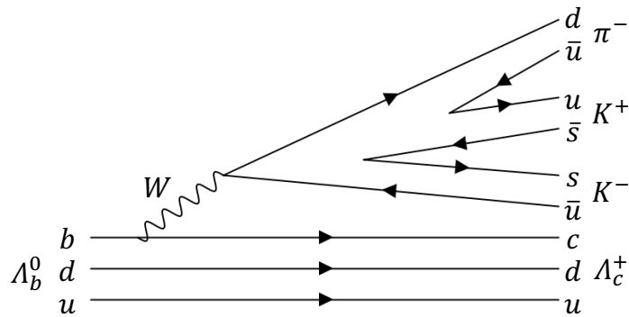
Figure 1: Feynman diagram of the leading contribution to the \Lambda_b^0 \rightarrow \Lambda_c^+ K^+ K^- \pi^- signal decay.
