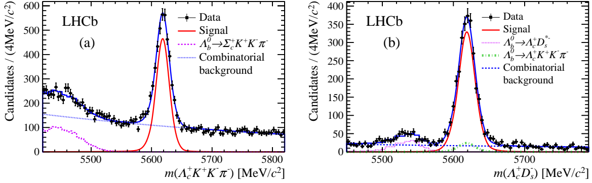
Figure 2: Invariant mass distribution of (a) \Lambda_b^0 \rightarrow \Lambda_c^+ K^+ K^- \pi^- and (b) \Lambda_b^0 \rightarrow \Lambda_c^+ D_s^- candidates. Fit projections are overlaid as a blue solid line. For (a), the red solid line represents the signal component, the blue dashed line is the background due to random combinations, and the violet dotted line is the contribution from \Lambda_b^0 \rightarrow \Sigma_c^+ K^+ K^- \pi^- decays. For (b), the red solid line is the normalization channel component, the violet dotted line is the \Lambda_b^0 \rightarrow \Lambda_c^+ D_s^{*-} background, the green dashed-dotted line is the contribution from \Lambda_b^0 \rightarrow \Lambda_c^+ K^+ K^- \pi^- decays, and the blue dashed line represents combinatorial background.
