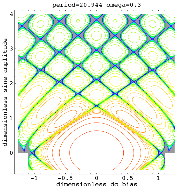
Figure 5: Phase-lock areas and their constrictions for \omega = 0.3 . Figure taken from [13, fig. 1e)]
