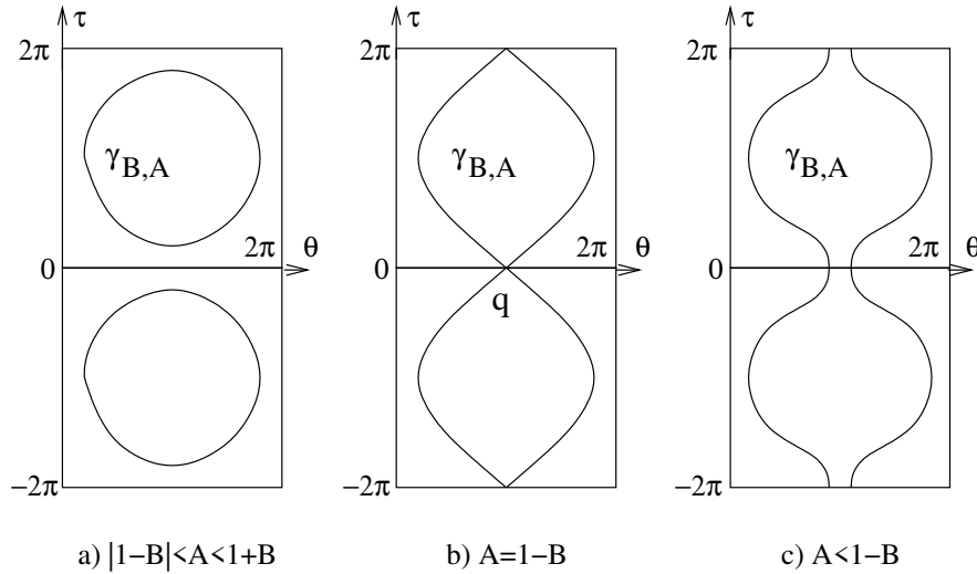
Figure 8: Different topological types of the curve \gamma_{B,A} = \{f(\theta, \tau) = 0\} for B, A > 0, A < 1 + B . We present its liftings to the universal covering \mathbb{R}^2_{\theta,\tau} .
