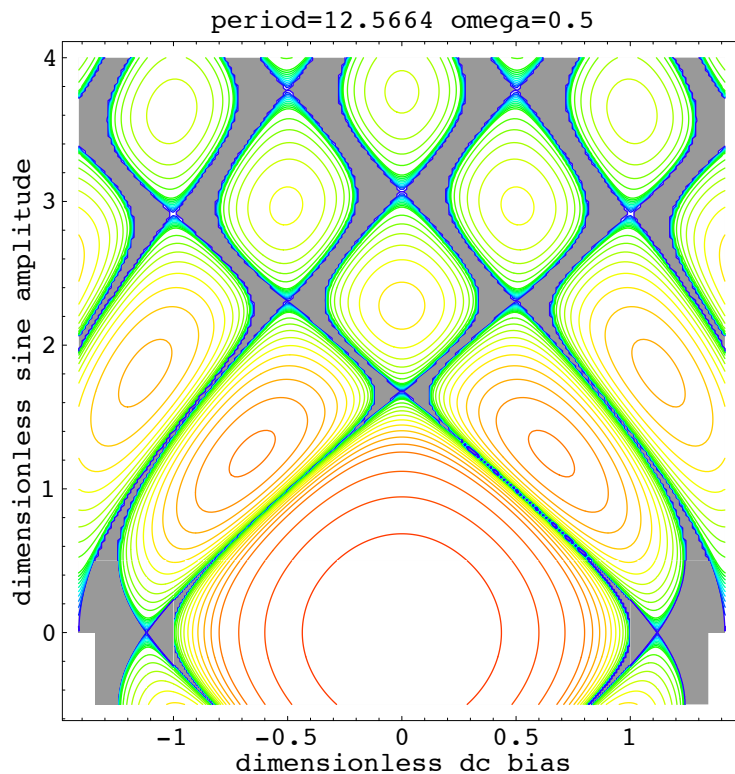
Figure 4: Phase-lock areas and their constrictions for \omega = 0.5 . Figure taken from [13, fig. 1d)]
