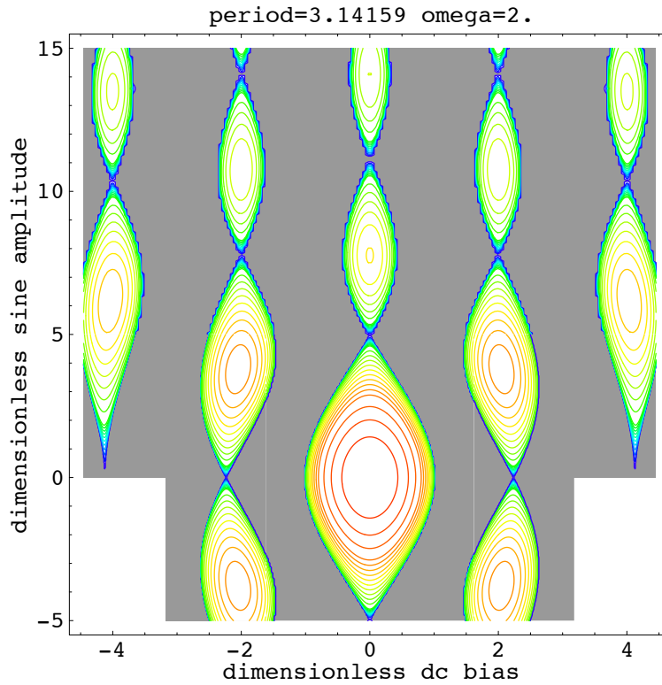
Figure 1: Phase-lock areas and their constrictions for \omega = 2 . The abscissa is B , the ordinate is A . Figure taken from [13, fig. 1a)]
