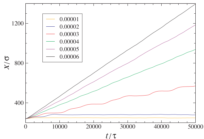
Fig. 5. The time dependence of the droplet center of mass for the indicated values of the external force, f_x (in units \epsilon/\sigma ). The interaction energy between sphere atoms and liquid monomers is \epsilon_{sp} = 0.6\epsilon .
