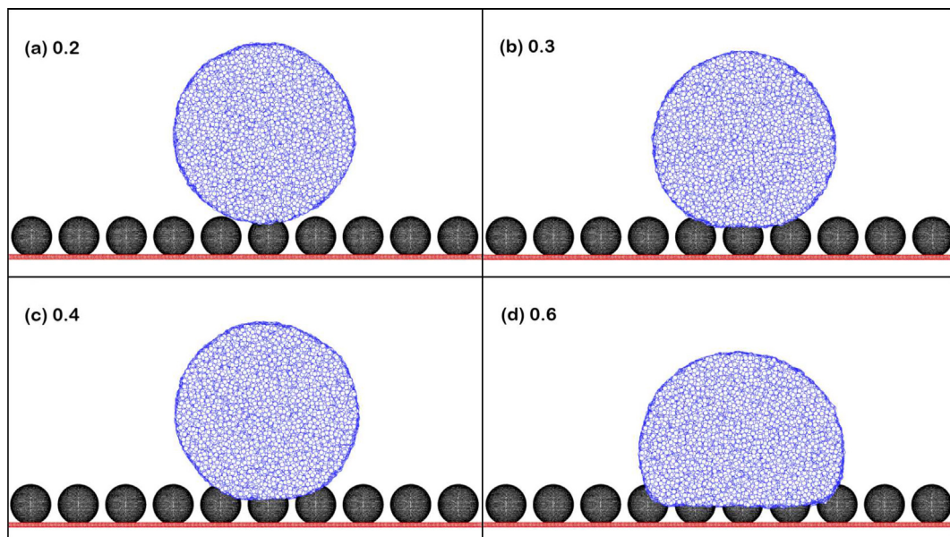
Fig. 2. The side view of polymer droplets in contact with solid particles for the surface energies (a) \epsilon_{sp} = 0.2\epsilon , (b) \epsilon_{sp} = 0.3\epsilon , (c) \epsilon_{sp} = 0.4\epsilon , and (d) \epsilon_{sp} = 0.6\epsilon .
