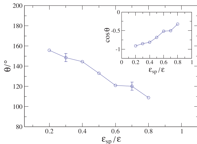
Fig. 4. The apparent contact angle for the droplet suspended on an array of spherical particles as a function of the interaction energy between sphere atoms and liquid monomers. The same data are replotted in the inset as \cos\theta(\epsilon_{sp}) .
