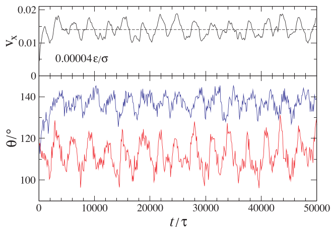
Fig. 7. The center of mass velocity (in units \sigma/\tau ) as a function of time when f_x = 0.00004\epsilon/\sigma (the upper panel). The dashed line denotes the average velocity v_x = 0.014\sigma/\tau . The interaction energy between sphere atoms and droplet monomers is \epsilon_{sp} = 0.6\epsilon . The time dependence of the advancing (blue curve) and receding (red curve) contact angles for f_x = 0.00004\epsilon/\sigma (the lower panel).
