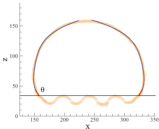
Fig. 3. An example of the droplet interface (orange circles) computed from the spatial variation of the local density profiles (see text for details) for \epsilon_{sp} = 0.6\epsilon and f_x = 0 . The horizontal black line denotes the reference plane above the tips of spherical particles. The blue curves indicate the 4-th order polynomial fit, and the red lines denote the local tangents to the polymer interface used to compute the apparent contact angles.
