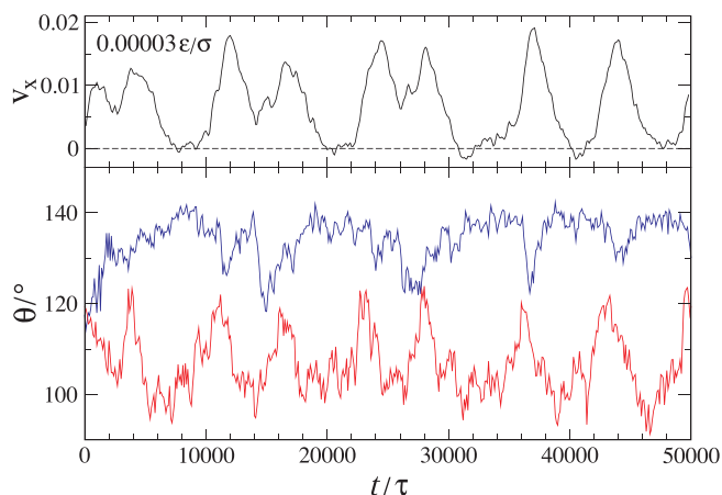
Fig. 6. The velocity of the center of mass (in units \sigma/\tau ) as a function of time when f_x = 0.00003\epsilon/\sigma (the upper panel). The horizontal dashed line indicates v_x = 0 . The advancing (blue curve) and receding (red curve) contact angles during 50000\tau (the lower panel). The surface energy is \epsilon_{sp} = 0.6\epsilon .
