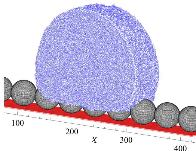
Fig. 1. An instantaneous snapshot of the liquid droplet that consists of 880 000 polymer chains (10 monomers per chain) and resides on the array of spherical particles rigidly attached to the solid substrate. The atoms are not shown to scale. The interaction energy between liquid monomers and particle atoms is \epsilon_{sp} = 0.6\epsilon . The external force f_x = 0.00004\epsilon/\sigma is applied on each monomer.
