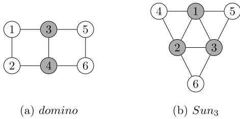
Fig. 1. Graphs (a) domino , and (b) Sun 3 .
