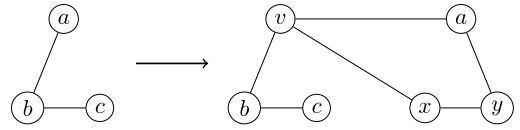
Fig. 2. Transformation \gamma(a, b) .
