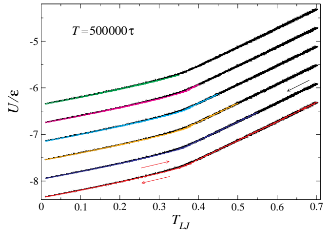
Fig. 5. The dependence of the potential energy during the thermal cycle with the period T = 500000\tau and the maximum temperature T_{LJ}^M = 0.35\epsilon/k_B (green), 0.40\epsilon/k_B (magenta), 0.45\epsilon/k_B (cyan), 0.50\epsilon/k_B (orange), and 0.55\epsilon/k_B (blue), and 0.70\epsilon/k_B (red). The potential energy during cooling with the rate 10^{-5}\epsilon/k_B\tau is indicated by the black curves. Note that the data for 0.35\epsilon/k_B \leq T_{LJ}^M \leq 0.55\epsilon/k_B are displaced for clarity.
