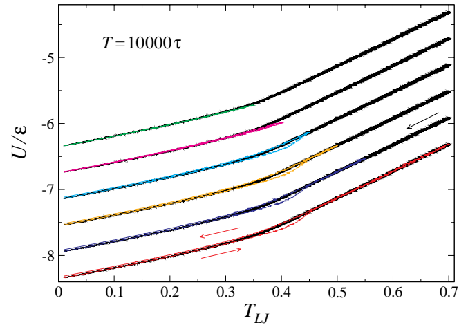
Fig. 4. The potential energy during heating and cooling with the period T = 10000\tau and the maximum temperature T_{LJ}^M = 0.35\epsilon/k_B (green), 0.40\epsilon/k_B (magenta), 0.45\epsilon/k_B (cyan), 0.50\epsilon/k_B (orange), and 0.55\epsilon/k_B (blue), and 0.70\epsilon/k_B (red). The black curves denote the potential energy during initial cooling with the rate 10^{-5}\epsilon/k_B\tau . All data, except for the two lowest curves (black and red), are displaced upwards for clarity.
