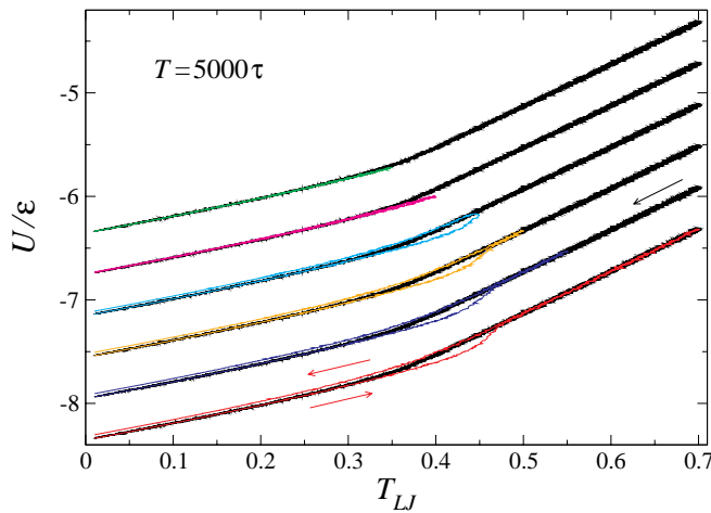
Fig. 3. The variation of the potential energy during one cycle with the period T = 5000\tau and the maximum temperature T_{LJ}^M = 0.35\epsilon/k_B (green), 0.40\epsilon/k_B (magenta), 0.45\epsilon/k_B (cyan), 0.50\epsilon/k_B (orange), and 0.55\epsilon/k_B (blue), and 0.70\epsilon/k_B (red). The black curves indicate the potential energy during cooling with the rate 10^{-5}\epsilon/k_B\tau . The data for 0.35\epsilon/k_B \leq T_{LJ}^M \leq 0.55\epsilon/k_B and the corresponding black curves are displaced vertically for clarity.
