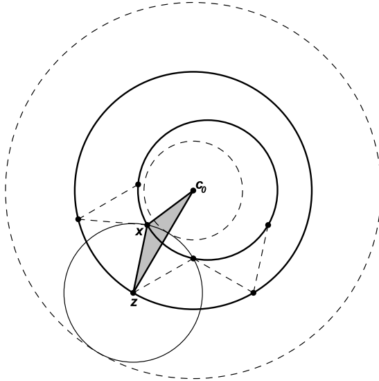
Figure 2: The invariant measure for the Zigzag theorem
