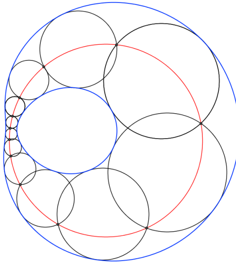
Figure 5: The Emch theorem for a cyclic
