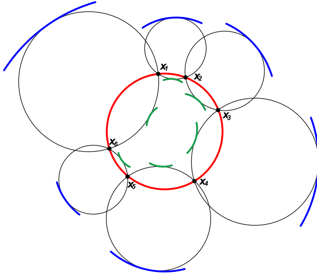
Figure 4: Emch theorem for pencils of circles
