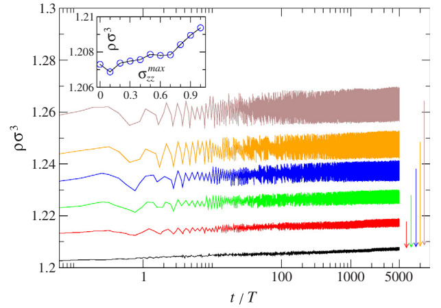
Fig. 4. The time dependence of the glass density, \rho\sigma^3 , during 5000 cycles for the stress amplitudes \sigma_{zz}^{\max}\sigma^3/\varepsilon = 0.0, 0.2, 0.4, 0.6, 0.8 , and 1.0 (from bottom to top). For clarity, the data are displaced vertically by +0.01\sigma^3 for \sigma_{zz}^{\max} = 0.2\varepsilon\sigma^{-3} (red), by +0.02\sigma^3 for \sigma_{zz}^{\max} = 0.4\varepsilon\sigma^{-3} (green), by +0.03\sigma^3 for \sigma_{zz}^{\max} = 0.6\varepsilon\sigma^{-3} (blue), by +0.04\sigma^3 for \sigma_{zz}^{\max} = 0.8\varepsilon\sigma^{-3} (orange), and by +0.055\sigma^3 for \sigma_{zz}^{\max} = 1.0\varepsilon\sigma^{-3} (brown). The vertical displacements of the data are marked by the arrows. The inset shows the average glass density after 5000 cycles as a function of the stress amplitude (see text for details). (For interpretation of the references to color in this figure legend, the reader is referred to the web version of this article.)
