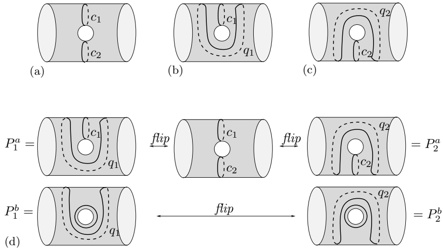
FIGURE 5. To the proof of Case 3.2.
