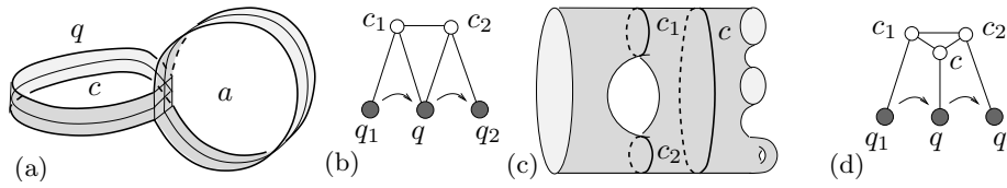
FIGURE 4. To the proof of Lemmas 4.6 and 4.9.
