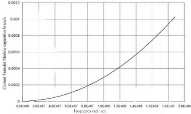
Fig. 4. Dependence of the gain module current in the capacitive branch of the signal frequency
