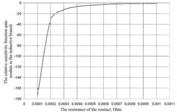
Fig. 6. Relative sensitivity function gain module current in the inductive branch of the value of active contact resistance
