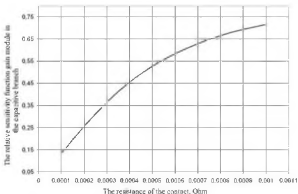
Fig. 8. Relative sensitivity function gain module from the current value of the active contact resistance
