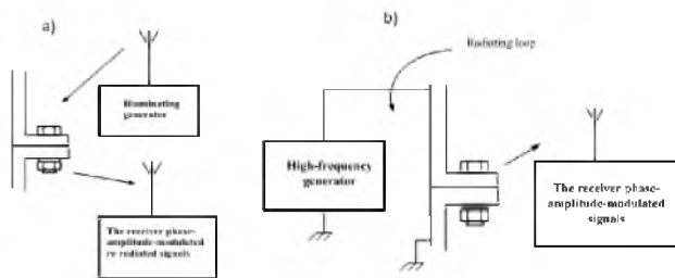
Fig. 2. Methods of obtaining information about the build quality: a - registration of the information about the parameters of re-emission signal; b - Check information about the parameters of the radiation signal
