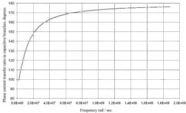
Fig. 5. Dependence of the phase current transfer ratio in the capacitive branch of the signal frequency
