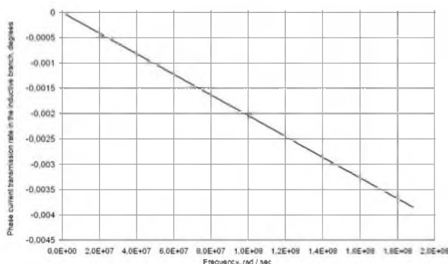
Fig. 3. Dependence of the phase current transfer ratio in the inductive branch of the signal frequency
