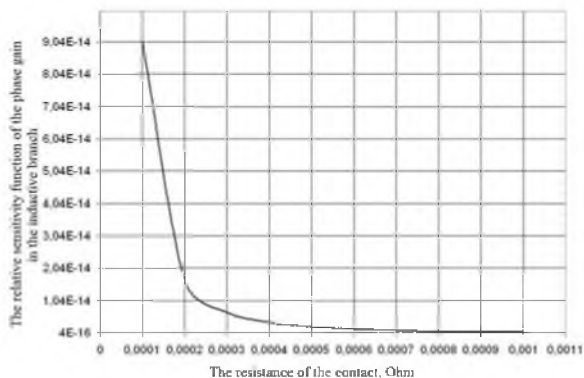
Fig. 7. Relative sensitivity function phase current transfer ratio in the inductive branch of the value of active contact resistance.
