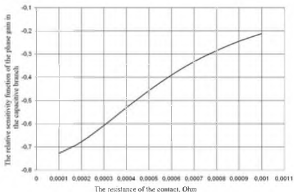
Fig. 9. Relative sensitivity function phase current transfer ratio in the capacitive branch of the value of active contact resistance
