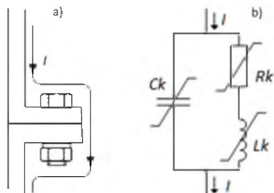
Fig. 1. Bolting (a) and the equivalent parametric variable impedance circuit contact (b)
