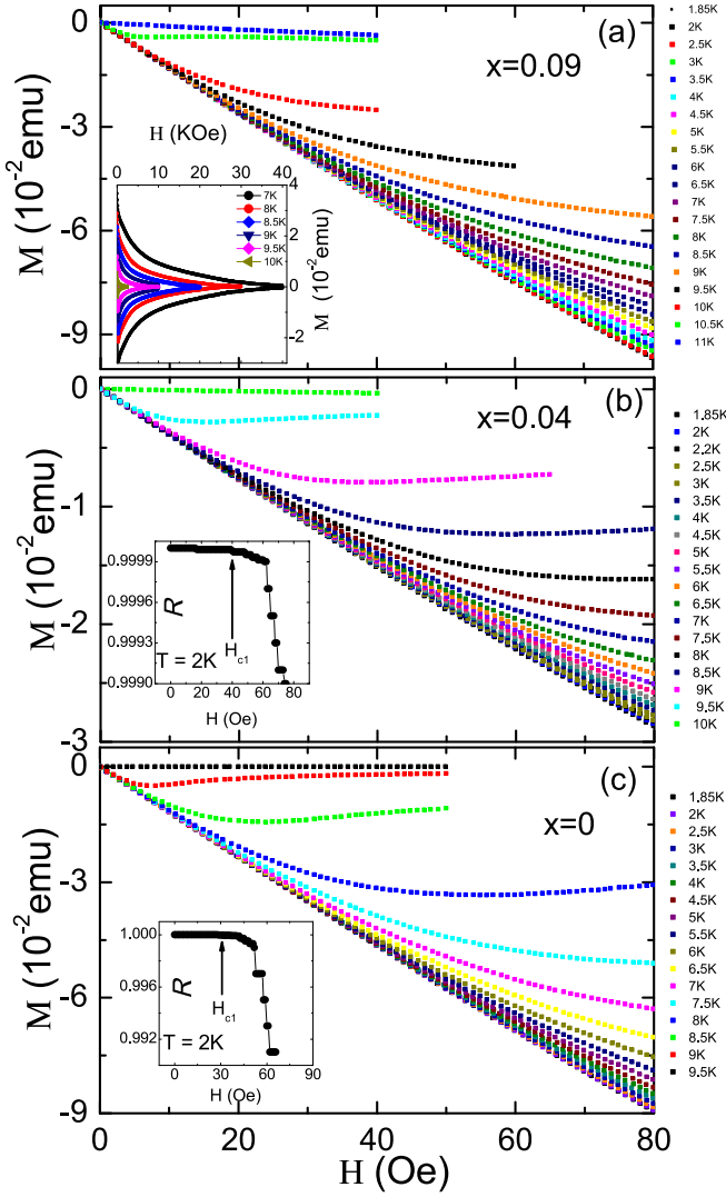
FIG. 5. (Color online) The field dependence of the initial diamagnetic part of the magnetization curves measured at various temperatures for H \parallel c in FeSe 1-x S x single crystal, for x = 0 , 0.04, and 0.09, respectively. The inset of (a) presents the magnetic field dependence of magnetization in FeSe 0.91 S 0.09 single crystal at different temperatures close to T_c . The insets in (b) and (c) depict an example used to determine the H_{c1} value using the regression factor R , at T = 2 K.
