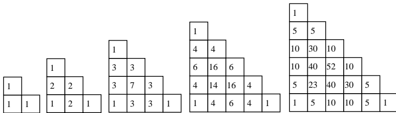
FIGURE 1. Triangular tables T^s containing the numbers V_{k,m}^s . South-west corners of these tables are located at (0, 0) .
