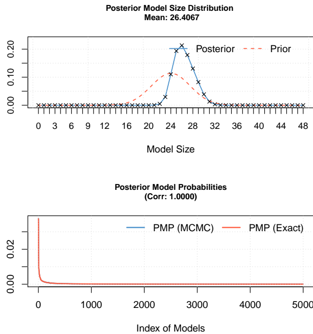
Figure A3: Model size and convergence, weights based on the number of estimates per study
