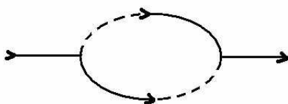
Figure 4. The graph defining \Sigma_{cl-cl} .
