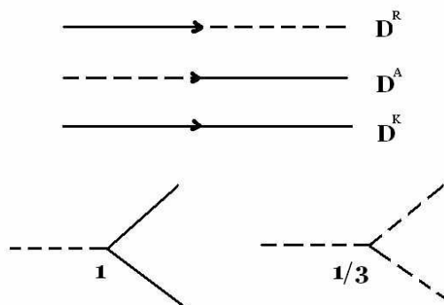
Figure 3. The solid line corresponds to \phi_{cl} , while the dashed line — to \phi_q .
