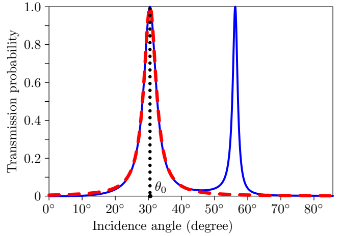
FIG. 10. Blue (solid) line: exact transmission probability for the symmetric n-p-n junction. Red (dashed bold) line: Lorenz–Breit–Wigner approximation p(\theta) \approx \frac{1}{1 + c(\theta - \theta_0)^2} .
