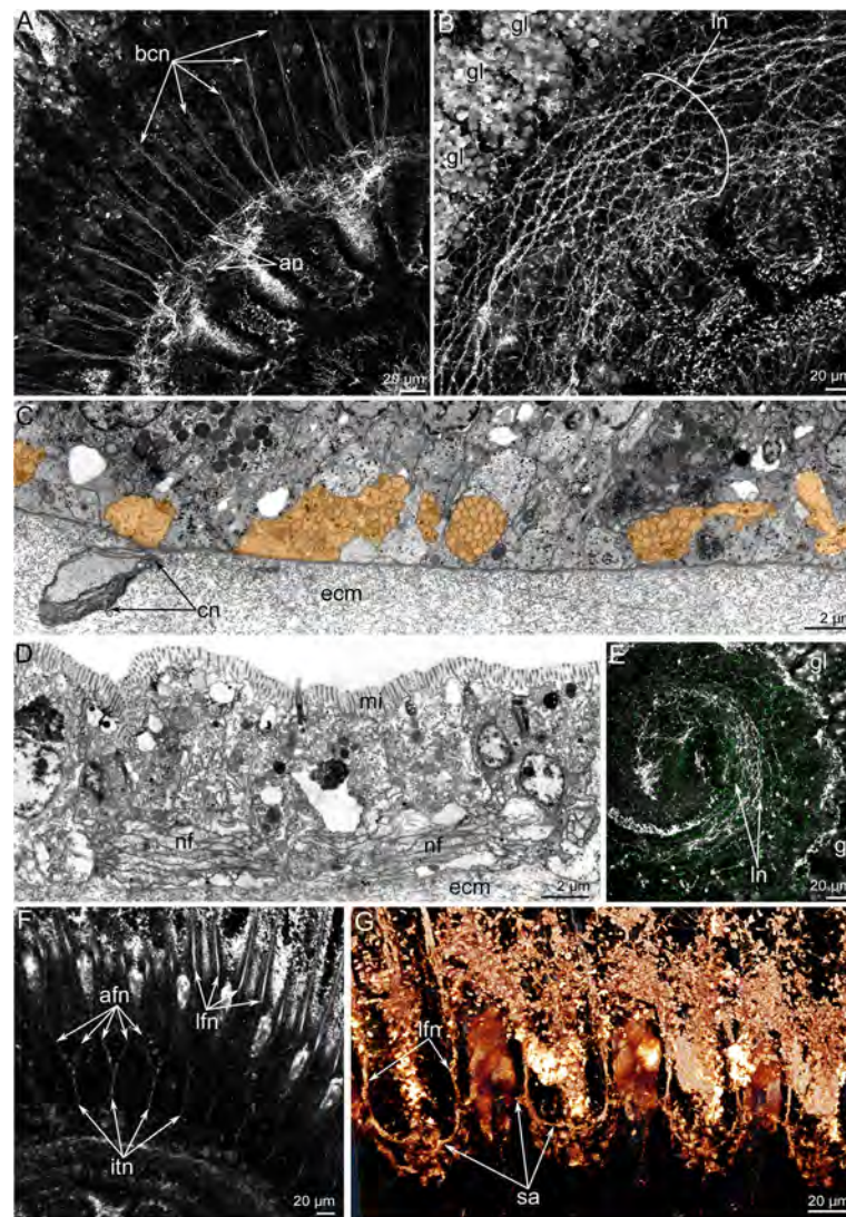
Fig. 9 Details of the organization of the accessory brachial nerve, the lower brachial nerve, and the second accessory nerve in Hemithiris psittacea . Z-projections after mono- (a, b) and double- (e) immunostaining against alpha acetylated-tubulin (grey) and serotonin (green); volume rendering of some nerve elements stained against alpha acetylated-tubulin (grey – f; glow – g): thin cross sections of the brachium (c-d). a The structure of the accessory brachial nerve appears disorganized. (B) The lower brachial nerve. c Ultrastructure of the accessory brachial nerve, which consists of several neurite bundles (marked by orange) scattered in the epithelium of the food groove. d Ultrastructure of the lower brachial nerve consisting of mostly longitudinal neurites. e The distal end of the brachium: a mesh of neurites of the lower brachial nerve (ln), which lacks a prominent serotonin-like immunoreactive portion. f Intertentacular nerves (itn) originate from the lower brachial nerve and give rise to the abfrontal tentacular nerves (afn) of outer tentacles. g A portion of the second accessory nerve (sa). Abbreviations: afn – abfrontal tentacular nerve; an – accessory brachial nerve; bcn – branches of cross nerves; ecm – extracellular matrix; gl – layer of glandular cells; itn – intertentacular nerve; lfn – laterofrontal tentacular nerve; ln – lower brachial nerve; mf – nerve fibers; mi – microvilli; sa – second accessory nerve
