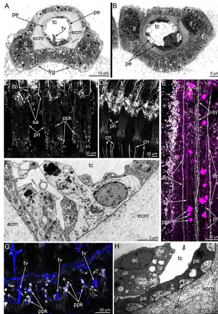
Fig. 4 Organization of tentacles in Hemithiris psittacea . Semi-thin cross sections ( a , b ); Z-projections after mono- ( c , d ) and double- ( e ) immunostaining against alpha acetylated-tubulin (grey) and serotonin (magenta); and staining with phalloidin (blue) ( g ); thin sections ( f , h ). a Outer tentacle. b Inner tentacle. c Z-projection of peritoneal nerves in outer tentacles. d Z-projection of peritoneal nerves in inner tentacles. e Z-projection of inner tentacle. f Cross section of the base of an outer tentacle: the large cell (ppk) with electron-lucent cytoplasm is visible. g Z-projection of the base of outer tentacles: perikarya of peritoneal cells (ppk) are visible. h Cross section of the lateral side of an inner tentacle: large peritoneal neurites (pn) contain electron-lucent cytoplasm. Abbreviations: ac – amoebocyte; af – abfrontal zone; cn – cross nerve; ecm – extracellular matrix; f – frontal zone; fn – frontal tentacular nerve; frg – frontal groove; lf – laterofrontal zone; lfn – laterofrontal tentacular nerve; pe – peritoneal cell of coelomic lining; pn – peritoneal neurite; ppk – peritoneal perikarya; sa – second accessory nerve; tc – tentacular coelom; tv – tentacular blood vessel
