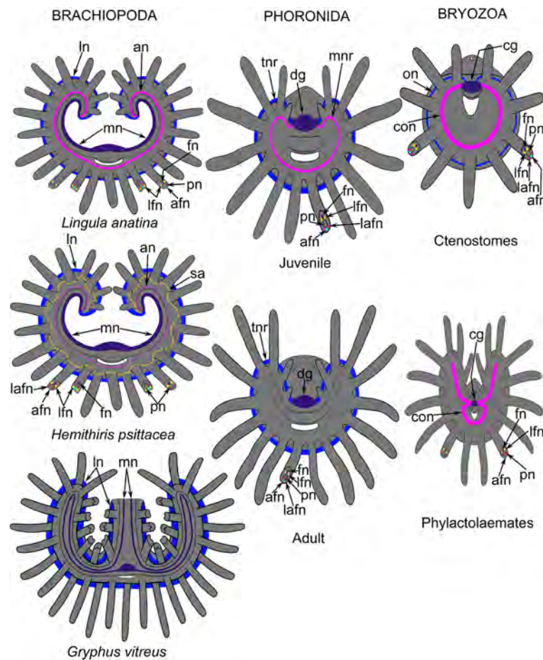
Fig. 12 Schemes of innervation of the lophophore in different brachiopods, phoronids, and bryozoans. Structures that are thought to be homologous are marked by the same color. Among brachiopods, the inarticulate Lingula anatina has three brachial nerves: main, accessory, and lower. The accessory nerve is well developed and contributes to innervation of tentacles. All tentacles are innervated by four tentacular nerves: abfrontal, two laterofrontal, and frontal. The scheme is based on [10]. The rhynchonelliform Hemithiris psittacea has four brachial nerves: main, accessory, second accessory, and lower. The accessory brachial nerve is poorly developed and does not contribute to the innervation of tentacles, whereas the lower brachial nerve is stronger and more prominent than in L. anatina . In H. psittacea , the outer tentacles are innervated by six tentacular nerves: abfrontal, two lateroabfrontal, two laterofrontal, and frontal. The scheme is based on this report. The rhynchonelliform Gryphus vitreus has two brachial nerves: main and lower. The tentacles are innervated by the lower brachial nerve, which is well developed. Details of tentacle innervation are not known; the scheme is based on [17]. Among phoronids, juveniles have oval-shaped lophophore, three nerve elements of the lophophore: dorsal ganglion (dg), minor nerve ring (mnr), and tentacular main nerve ring (tnr), whereas adults have horseshoe-shaped lophophore and lack the minor nerve ring. In all phoronids, tentacles are innervated by six tentacular nerves: abfrontal, two lateroabfrontal, two laterofrontal, and frontal. Scheme of juvenile lophophore is based on [30]; scheme of adult lophophore is based on [31, 37]. Among bryozoans, ctenostome bryozoans have the cerebral ganglion (cg), circumoral nerve ring (con), and outer nerve ring (on), whereas many other bryozoans (i.e. phylactolaemates) lack the outer nerve ring. In bryozoans, tentacles are innervated by four tentacular nerves: abfrontal, two laterofrontal, and frontal. The scheme of ctenostome lophophore is based on [11]; the scheme of phylactolaemates is based on [33, 49]. Abbreviations: afn – abfrontal tentacular nerve; an – accessory brachial nerve; cg – cerebral ganglion; con – circumoral nerve ring; dg – dorsal ganglion; fn – frontal tentacular nerve; lafn – lateroabfrontal tentacular nerve; lfn – laterofrontal tentacular nerve; ln – lower brachial nerve; mn – main brachial nerve; mnr – minor nerve ring; pn – peritoneal neurite; sa – second accessory brachial nerve; tnr – tentacular main nerve ring
