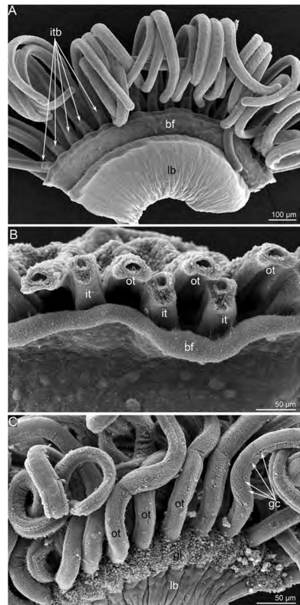
Fig. 2 Details of lophophore organization in Hemithiris psittacea ; SEM. a A portion of the lophophore brachium, viewed from the brachial fold. b Two rows of tentacles (inner and outer) and the brachial fold, viewed from the top. c The base of the lophophore arm, viewed from the outer side. The layer of glandular cells is visible (gl). Abbreviations: bf – brachial fold; gc – openings of glandular cells along the lateroabfrontal side of tentacle; gl – layer of glandular cells at the base of the outer side of the lophophore; it – inner tentacle; itb – swollen base of inner tentacles; lb – lophophore base; ot – outer tentacle
