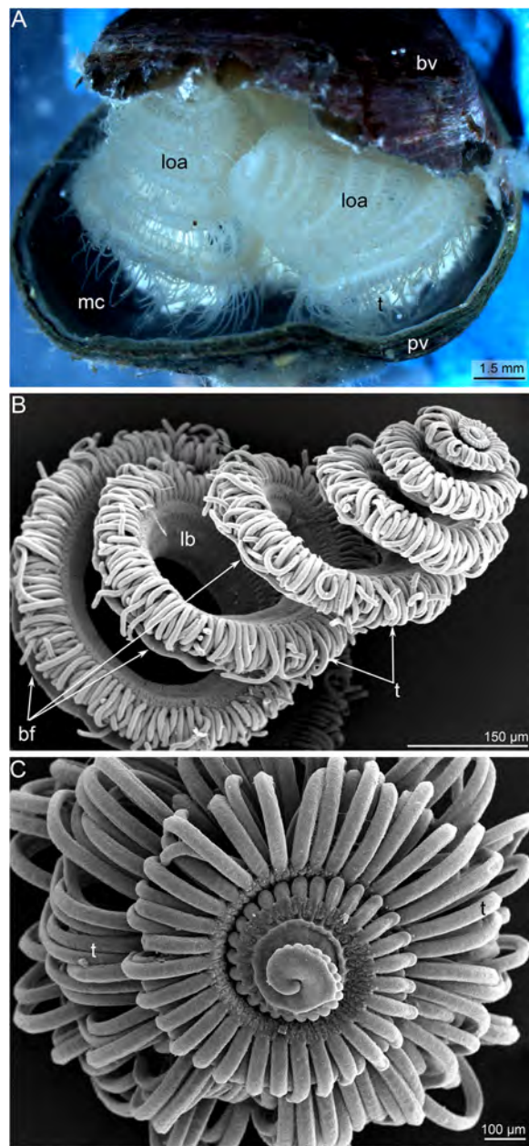
Fig. 1 Organization of the lophophore in Hemithiris psittacea . a Photograph of a live animal: the brachial valve (bv) is broken. Two arms of the spirolophore lophophore are visible. b A brachium; SEM; lateral view. c The distal end of the brachium with the youngest tentacles; SEM; top view. Abbreviations: bf – brachial fold; bv – brachial valve of shell; lb – lophophore base; loa – lophophore arm (brachium); mc – mantle cavity; pv – pedal valve of shell; t – tentacle
