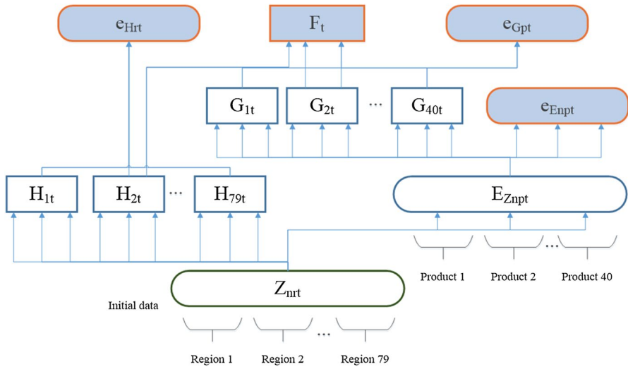
Fig. 3 Data blocks in the dynamic hierarchical factor model
