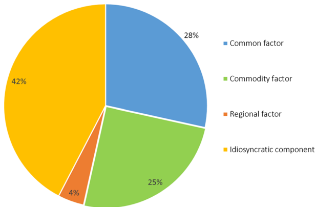
Fig. 13 Decomposition of variance of the aggregate inflation rate obtained under an alternative model's specification
