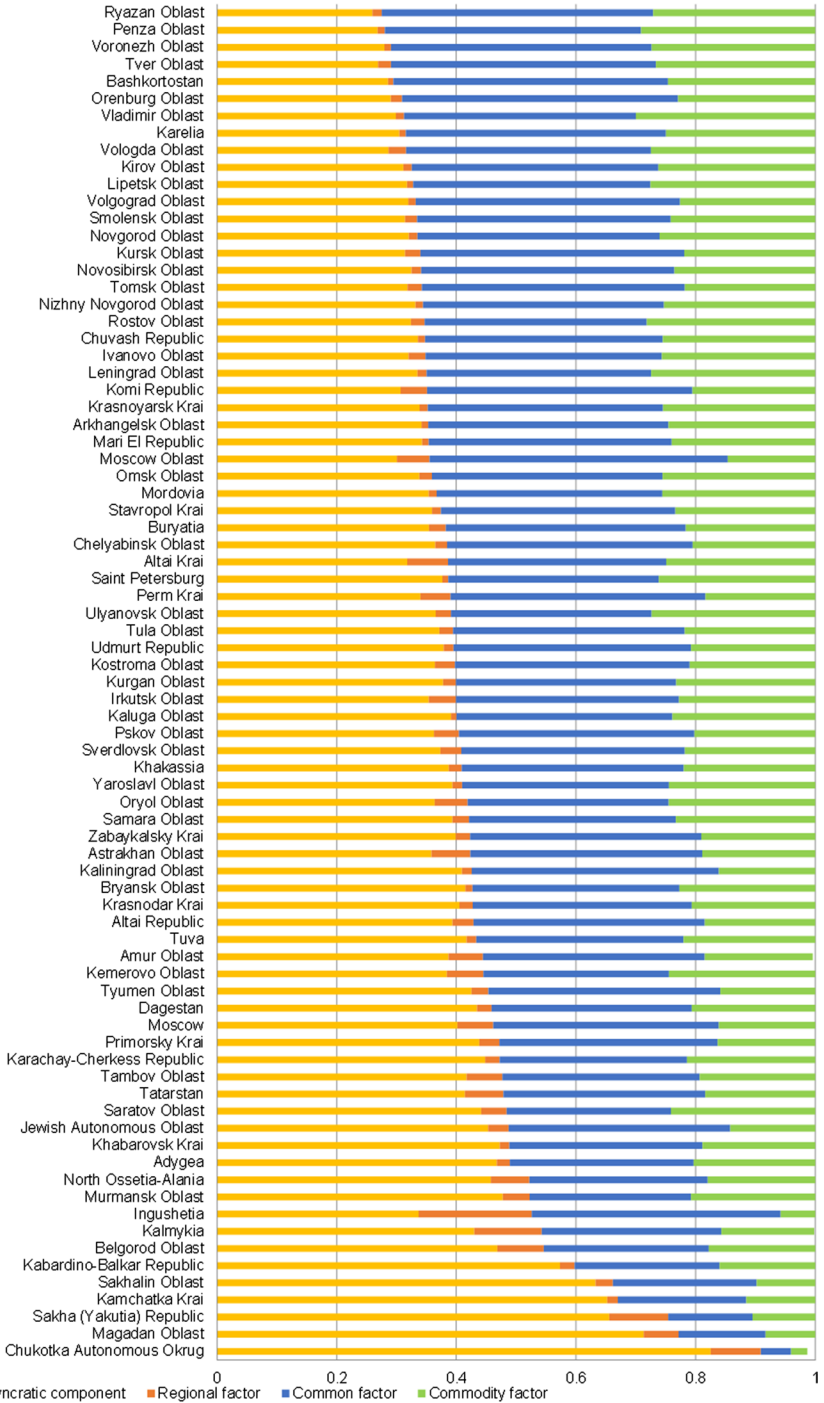
Fig. 7 Variance decomposition of inflation across regions ranked by the sum of regional and idiosyncratic components
