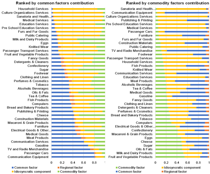
Fig. 5 Variance decomposition of inflation across commodities
