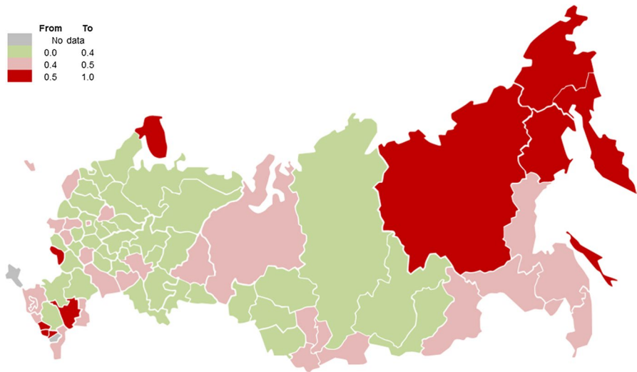
Fig. 8 Variance decomposition of inflation across regions (share of variance explained by regional and idiosyncratic components)
