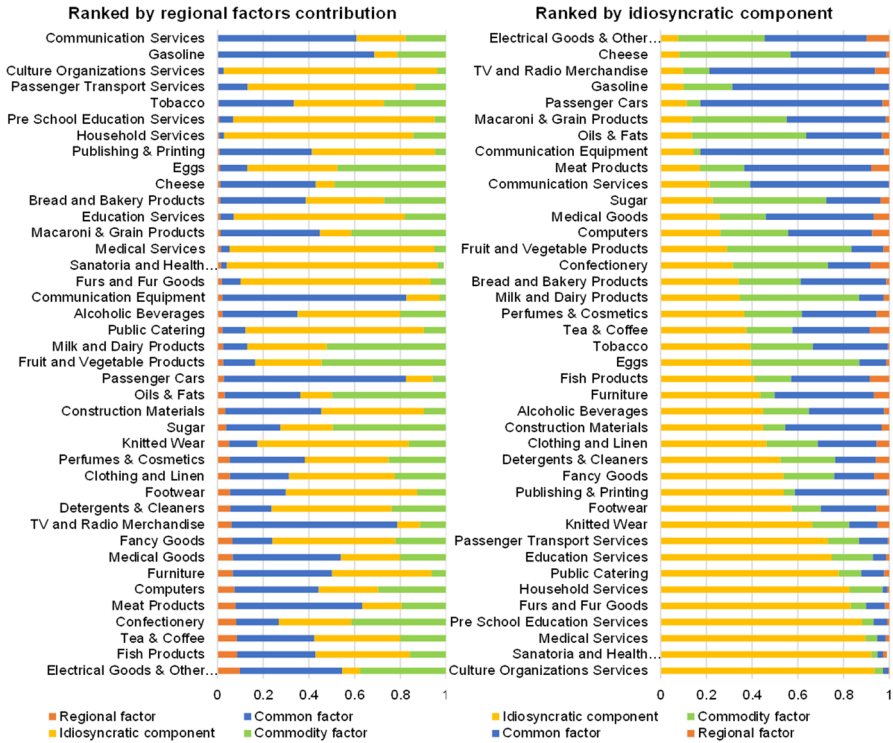
Fig. 6 Variance decomposition of inflation across commodities
