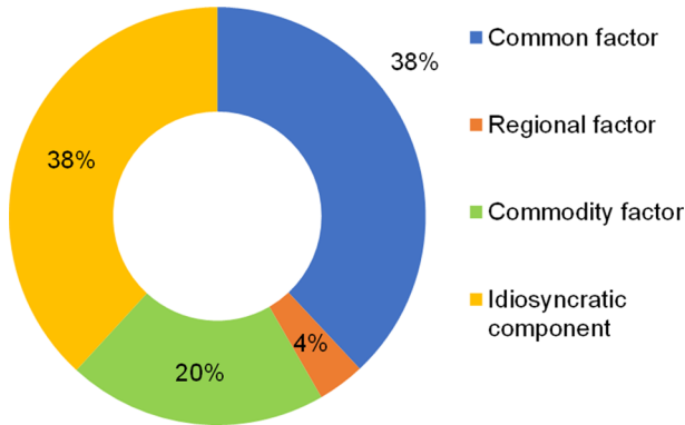
Fig. 4 Decomposition of variance of the aggregate inflation rate
