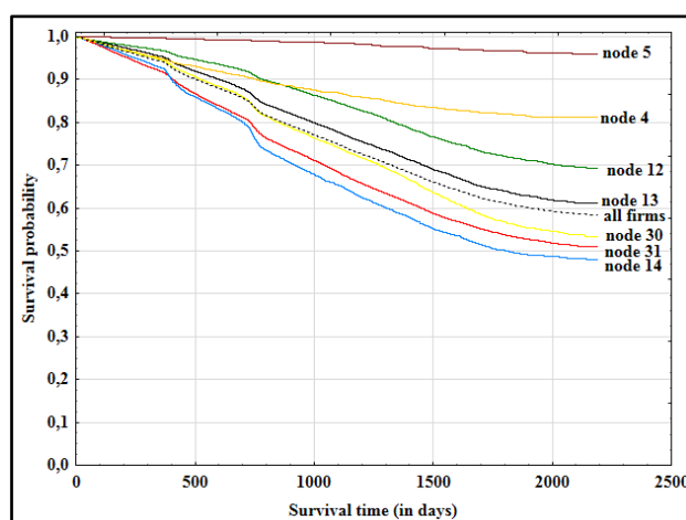
Fig. 2. The Kaplan-Meier survival curves for all data and 7 groups of enterprises separated in the leaves of the GUIDE tree.
