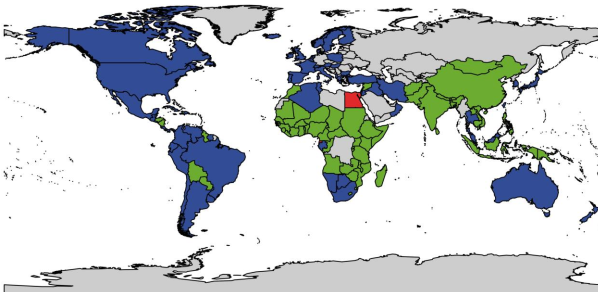
Fig. 5. Two rules of Table 1 classify countries in blue and green. For grey countries, no data was available in (Leister, 2016). The rules result from the clustering of Fig. 1. In red are the Outlier Equatorial Guinea as well as the incorrectly classified countries Egypt and Micronesia by these two rules.
