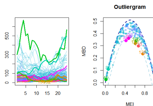
Fig. 8. Outliergram and outliers in air pollution data.
