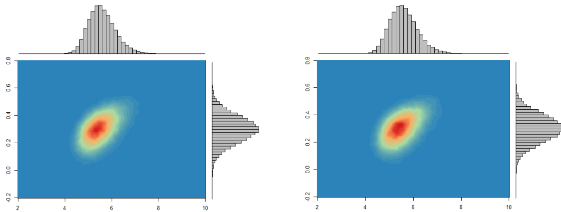
Fig. 1. The posterior distribution of (\varphi, \nu) in the EMSF-SBEKK model (exchange rates, T=1482 ; left panel: \lambda_v = 1/10 ; right panel: \lambda_v = 1/30 ).
