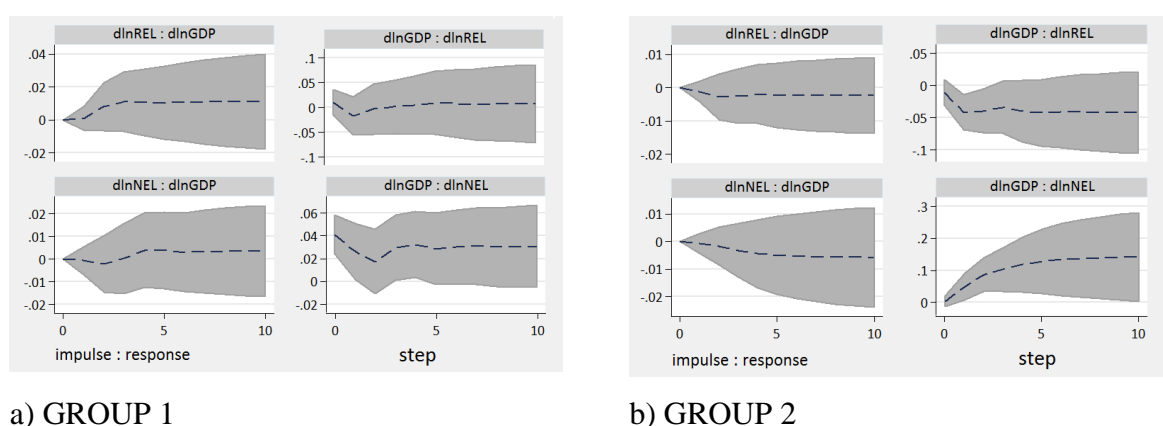
Fig. 1. Impulse response functions for the countries belonging to GROUP 1 or GROUP 2.
