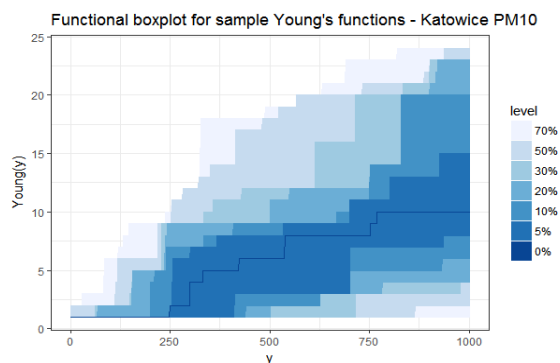
Fig. 6. Functional boxplot for Young inverse functions of air pollution curves in Katowice in 2016.
