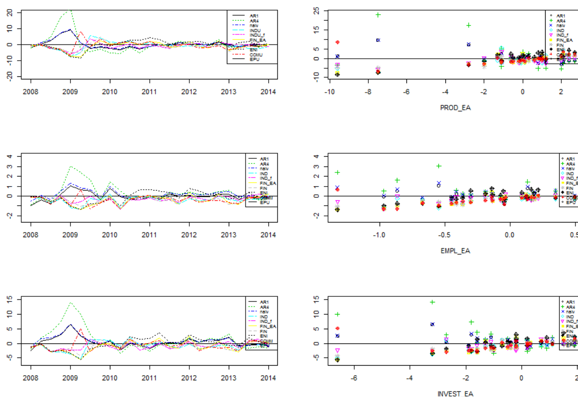
Fig.2 Forecast errors and the relations between the difference of macroeconomic variables and forecast errors.
