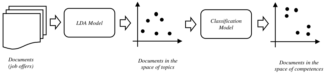
Fig. 1. The structure of the model mapping job offers into the space of competences.
