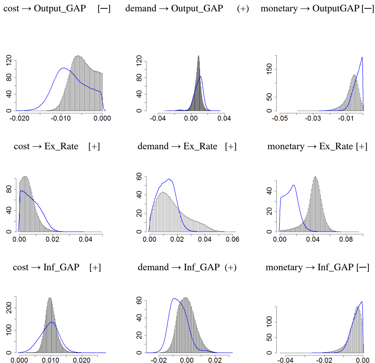
Fig. 1. Marginal posteriors (histograms) and priors (lines) of the elements of the instantaneous reactions matrix ( B ) obtained within the second model.
