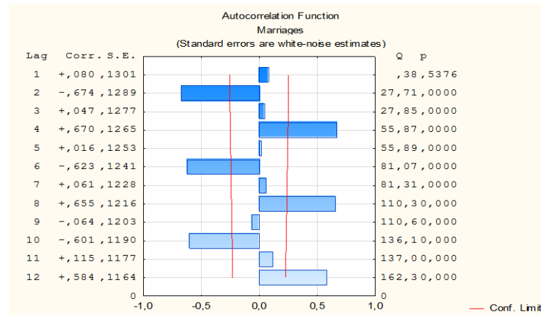
Fig. 3. Correlogram of the number of registered marriages.
