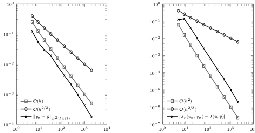
FIGURE 5. Example 2: errors as h refines and M = 2^{10}
