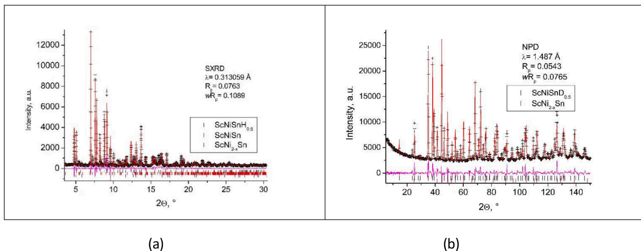
Fig. 3. (a) Rietveld refinement of the synchrotron X-ray powder diffraction pattern measured at 295 K. 2 theta angle range was 3.465-30.375°; Step size 0.005°; λ = 0.313059 Å. Experimental data: points; calculated data: line; residual intensities plot: bottom line. Positions of the peaks are shown by ticks; ScNiSnH 0.5 – top; ScNiSn – middle; ScNi 2-x Sn – bottom. (b) Rietveld profile fit of the neutron powder diffraction pattern of ScNiSnD 0.5 (λ = 1.487 Å) at 295.0 K. Experimental data: points; calculated data: line; residual plot: bottom line. Positions of the peaks are shown by ticks; ScNiSnD 0.5 – top; ScNi 2-x Sn – bottom.
